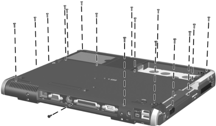
Torx T8M2.0×6.0 Screw Locations
