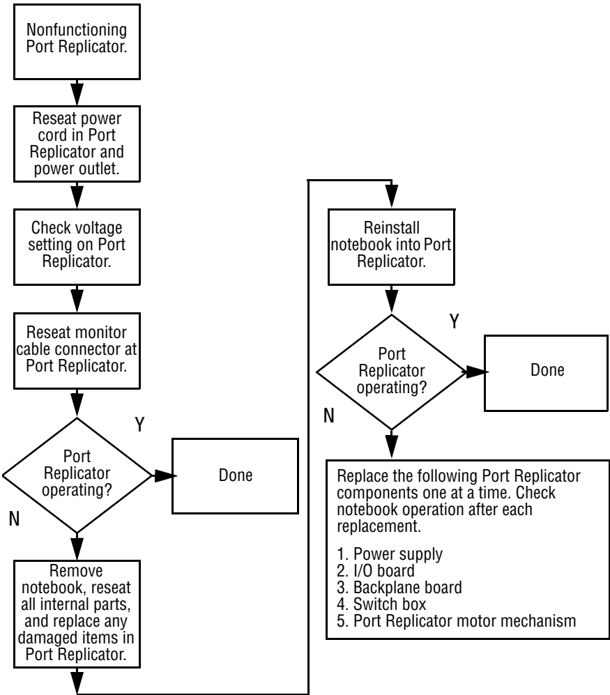
Flowchart 2.8—Nonfunctioning Port Replicator
