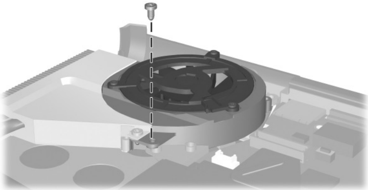
Torx T8M2.0×4.0 Screw Location
