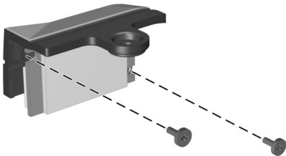
Phillips PM1.5×3.0 Screw Locations
