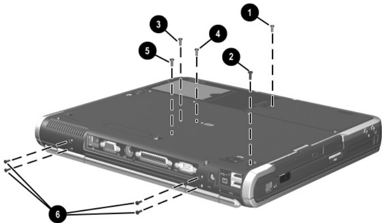
Torx T8M2.0x6.0 Screw Locations
