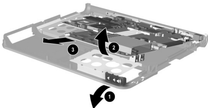
Removing the System Board
