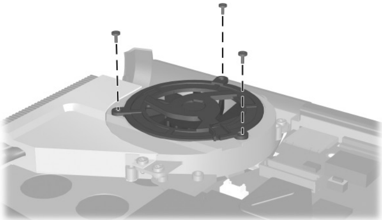
Phillips PM1.5×4.0 Screw Locations
