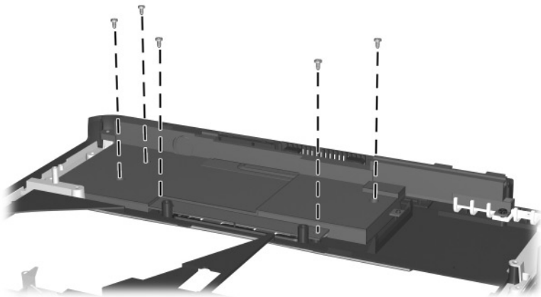
Torx T8M2.0×4.0 Screw Locations
